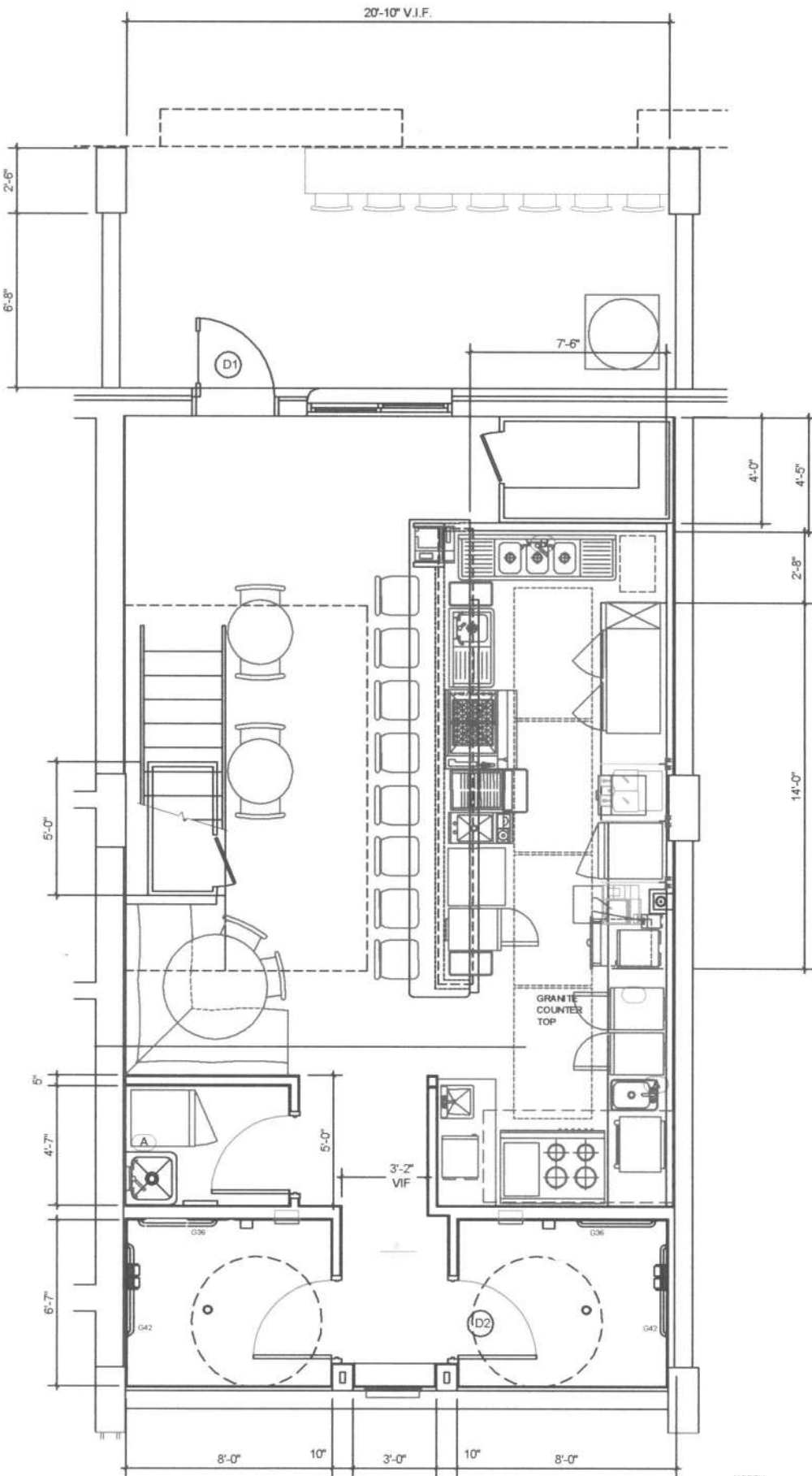
1 FLOOR PLAN-ARCHITECTURAL A1.1 ENTRY LEVEL 3/8"=1'-0"
